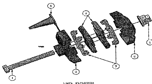
VISTA EXPLODIDA
